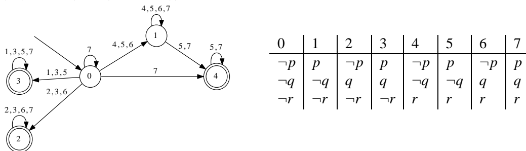
Figure 5: LTL formula together with its minimal automaton and the boolean value to alphabet translation table
